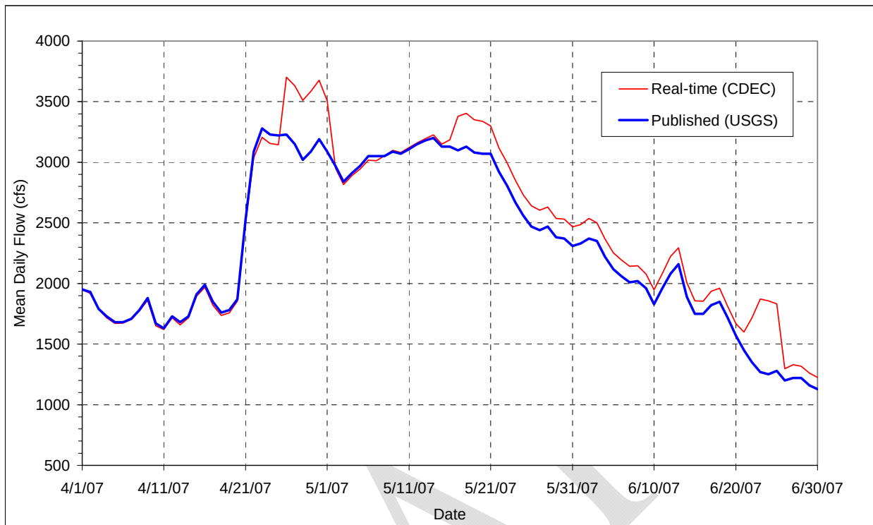
Figure 5 Comparison of Real-time and Published Flow Data, San Joaquin River near Vernalis
